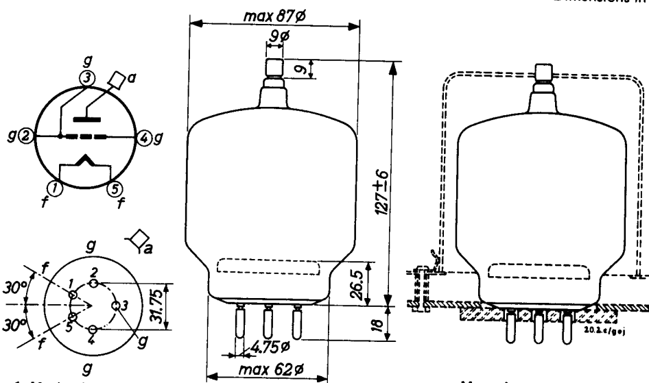
Fig. 1 Mechanical outline.
